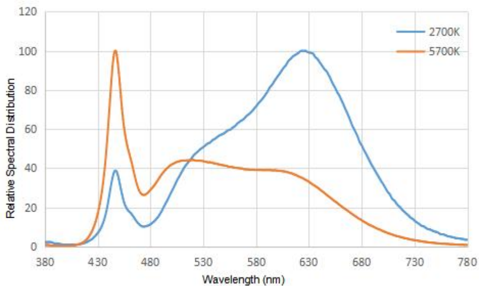
Figure 1a. Typical normalized power vs. wavelength for at test current, RA90 T_j = 25^\circ \text{C} .
