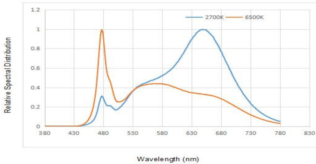
Figure 1a. Typical normalized power vs. wavelength for at test current, RA90 Tj =25° C.
