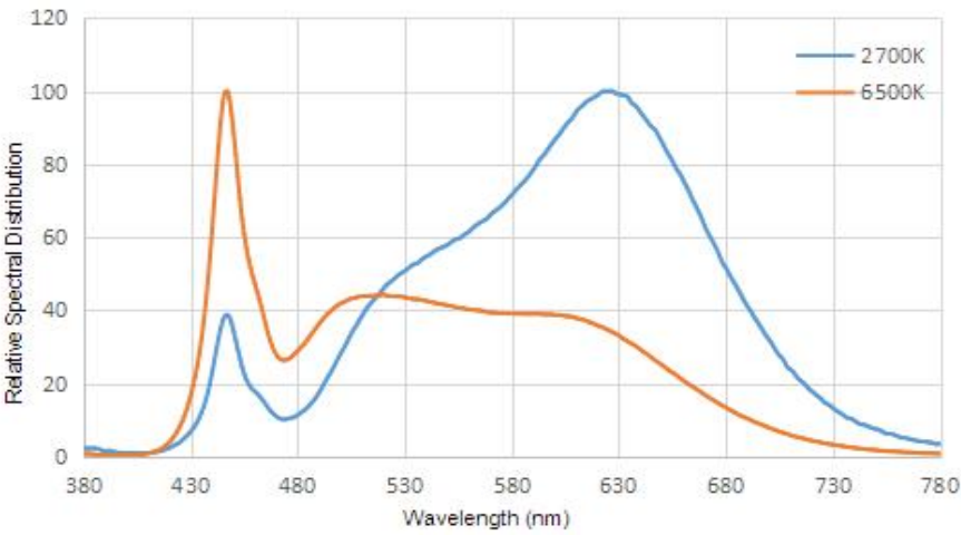
Figure 1a. Typical normalized power vs. wavelength for at test current, RA95 Tj =25° C.
