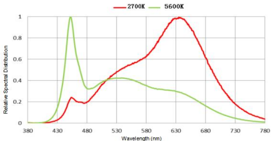
Figure 1a. Typical normalized power vs. wavelength for at test current, RA95 Tj =25° C.
