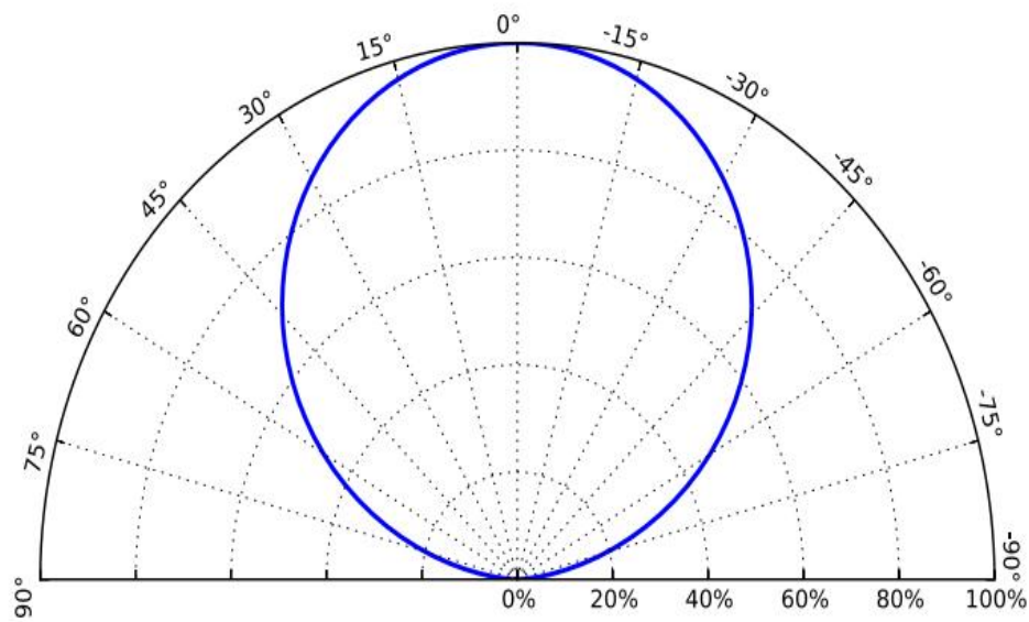
Typical radiation pattern for T at test current, T_j = 25^{\circ}\text{C} .
